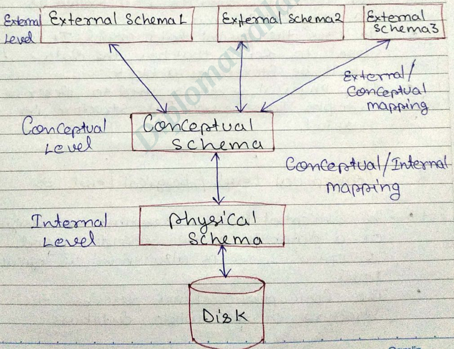
Three-Schema Architecture.
